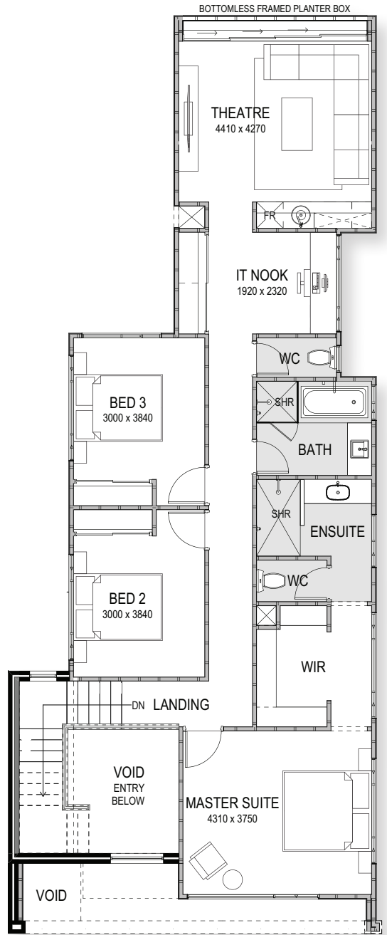
FIRST FLOOR
