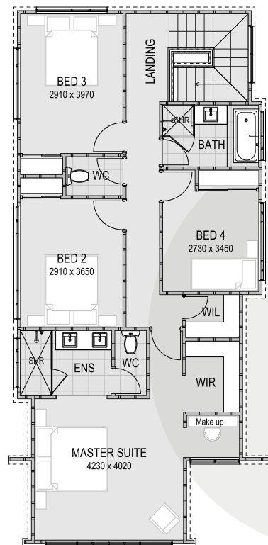
UPPER FLOOR
