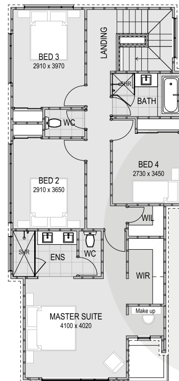
UPPER FLOOR
